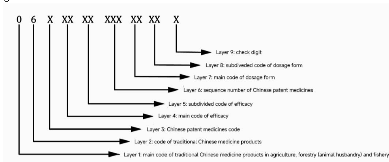
Figure 1 Coding structure of Chinese patent medicines
